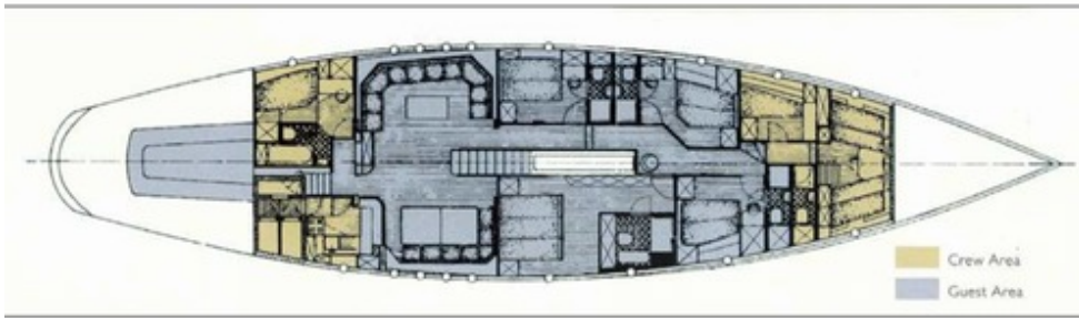
General Arrangement
